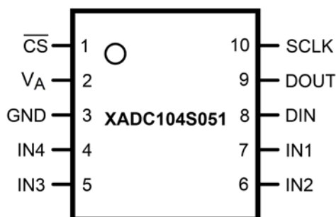
Figure 2. Pin Configuration
