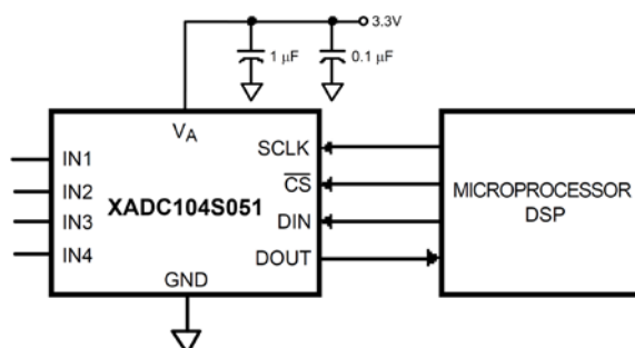
Figure 3. Typical Circuit Configuration
