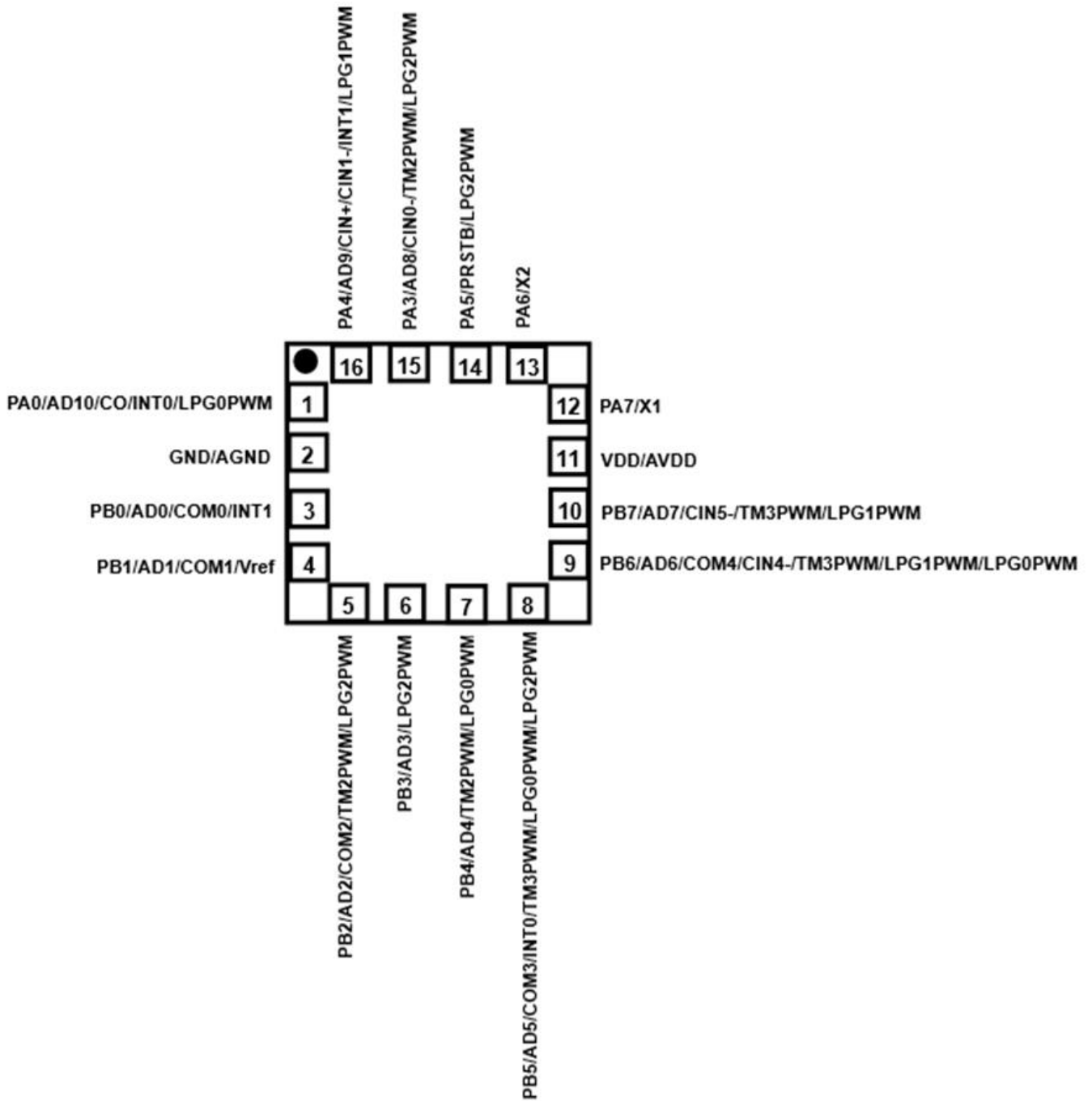
PFS123B-1J16A: QFN3*3-16P (0.5pitch)
