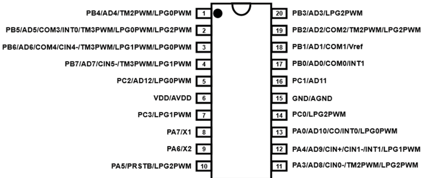
PFS123B-S20A: SOP20 (300mil) PFS123B-H20A: HTSOP20 (150mil)
