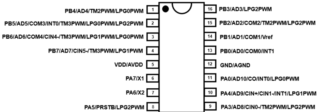
PFS123B-S16A: SOP16 (150mil)
