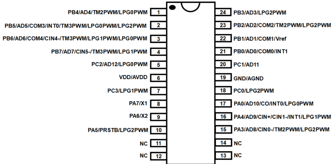
PFS123B-Y24A: SSOP24 (150mil)
