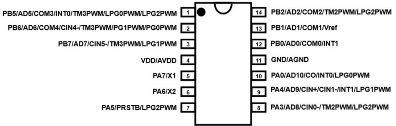
PFS123B-S14A: SOP14 (150mil)
