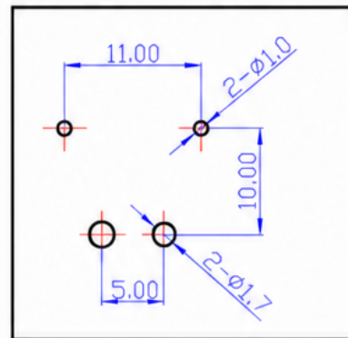
Mounting Hole Diagram
