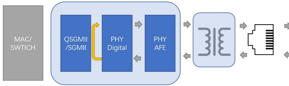
Figure 11. Remote PHY Loopback
