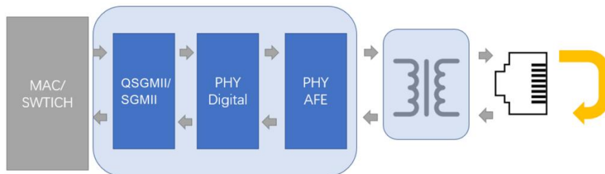
Figure 10. External Loopback
