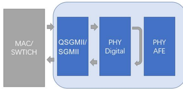
Figure 9. Digital Loopback
