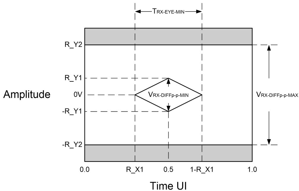
Figure 17. 1000BASE-X Differential Receiver Eye Diagram
