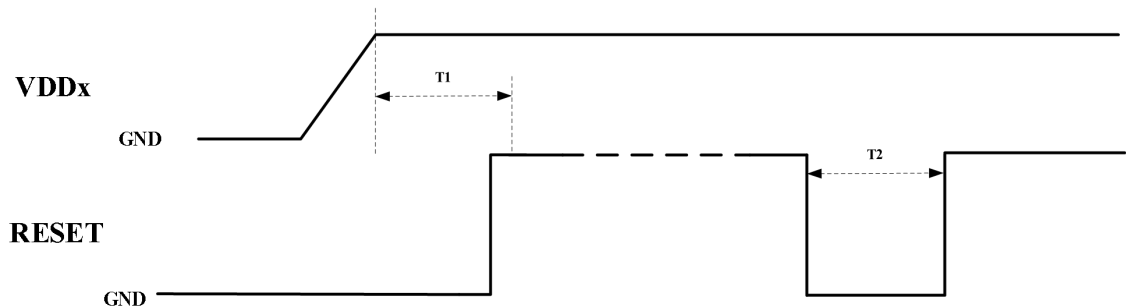
Figure 8. Reset Timing Diagram
