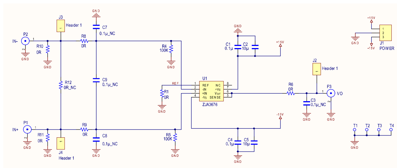
Figure 51. ZJA3676 Evaluation Board Schematic
