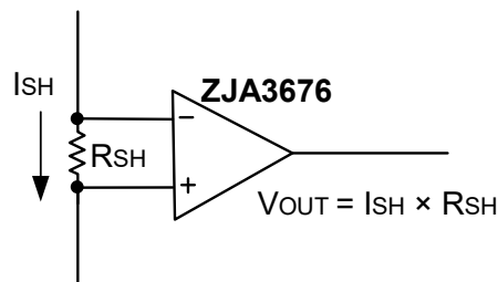
Figure 49. ZJA3676 Monitoring Current Through a Shunt Resistor
