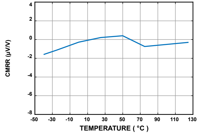
Figure 9. CMRR vs. Temperature
