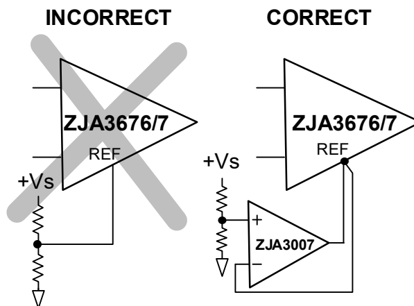
Figure 39. Driving the REF Pin
