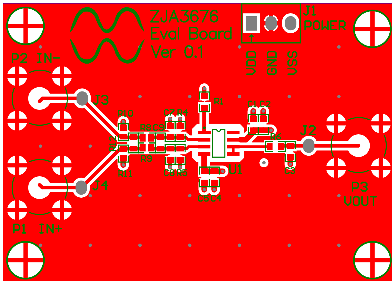
Figure 52. Layout of ZJA3676 Evaluation Board (Top Layer)
