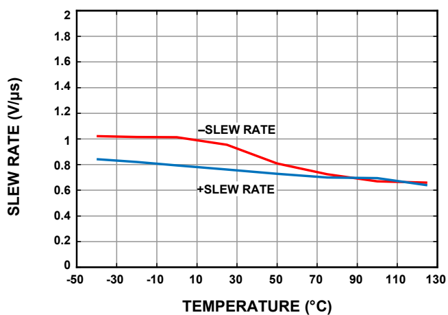
Figure 24. Slew Rate vs. Temperature ( V_{IN} = 20 V_{P-P} , 1 kHz)
