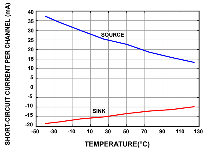
Figure 23. Short-Circuit Current per Channel vs. Temperature
