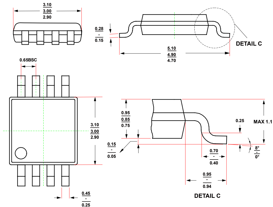
Figure 55. 8-Lead MSOP Package Dimensions shown in millimeters
