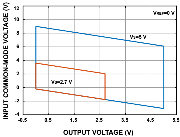
Figure 18. Input Common-Mode Voltage vs. Output Voltage (5 V and 2.7 V Supplies, V_{REF} = 0 V)
