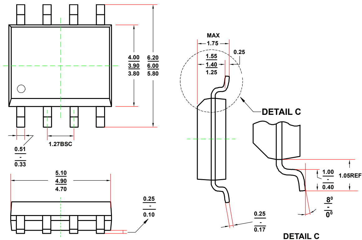
Figure 54. 8-Lead SOIC Package Dimensions shown in millimeters
