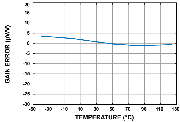
Figure 11. Gain Error vs. Temperature
