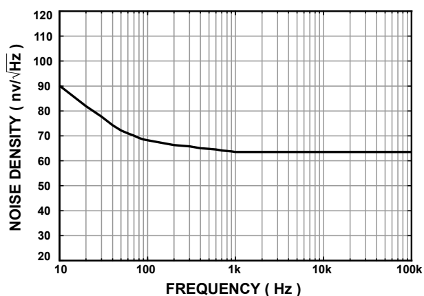
Figure 34. Voltage Noise Density vs. Frequency
