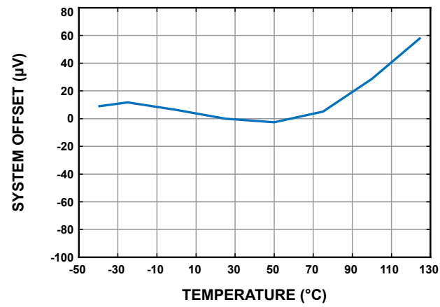
Figure 7. System Offset vs. Temperature, Normalized at 25 °C
