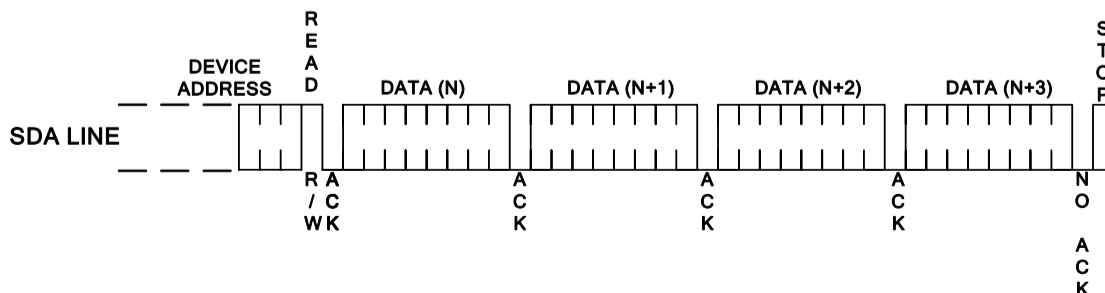
Figure 6: Sequential Read
