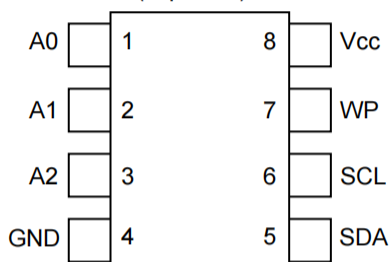
8-lead DIP/SOP/MSOP/TSSOP (Top View)
