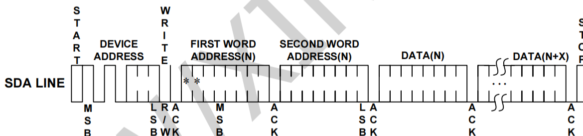
Figure 4: Page Write
