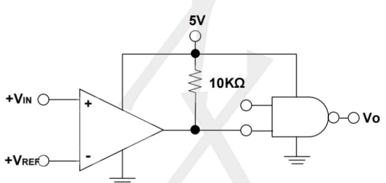
Driving CMOS/TTL
