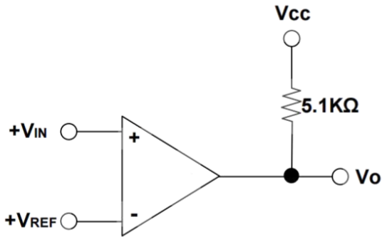
Basic Comparator
