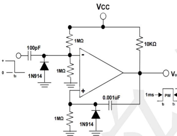
One-Shot Multivibrator
