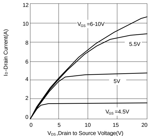
Figure 10: Output Characteristics
