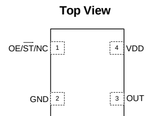
Figure 1. Pin Assignments
