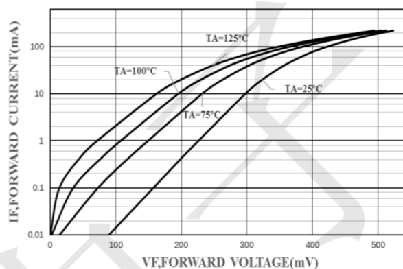
FIG 2.TYPICAL FORWARD CHARACTERISTIC
