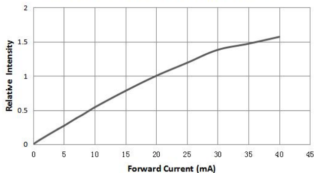
Relative Intensity VS. Forward Current ( T_a=25^{\circ}\text{C} )
