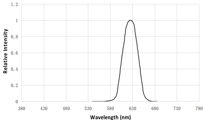
Spectrum Distribution ( T_a=25^{\circ}\text{C} )
