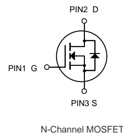
TO-252-2L (TO-252(DPAK))
