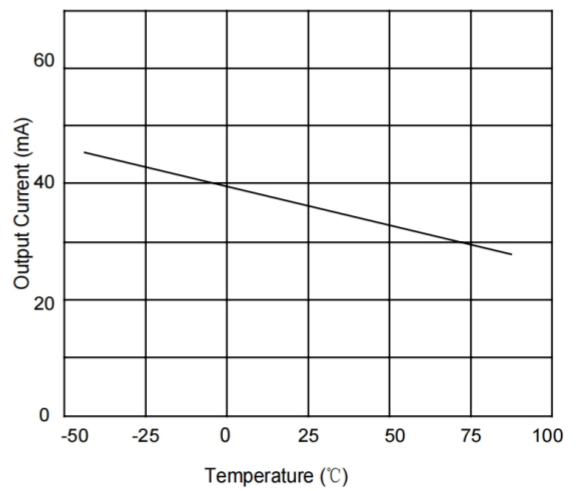
Fig.12 Current Limiting
