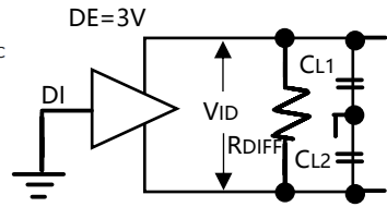
Figure 3 Driver switch characteristic test circuit
