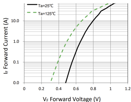
Figure 1. Forward Characteristic(typ.)
