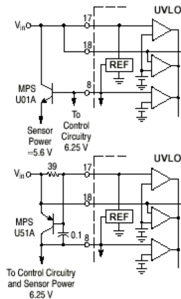
Figure 21. Reference Output Buffers
