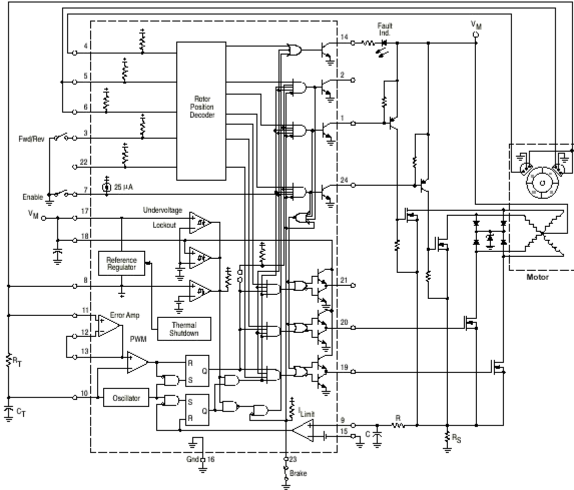
Figure 44. Four Phase, Four Step, Half Wave Motor Controller
