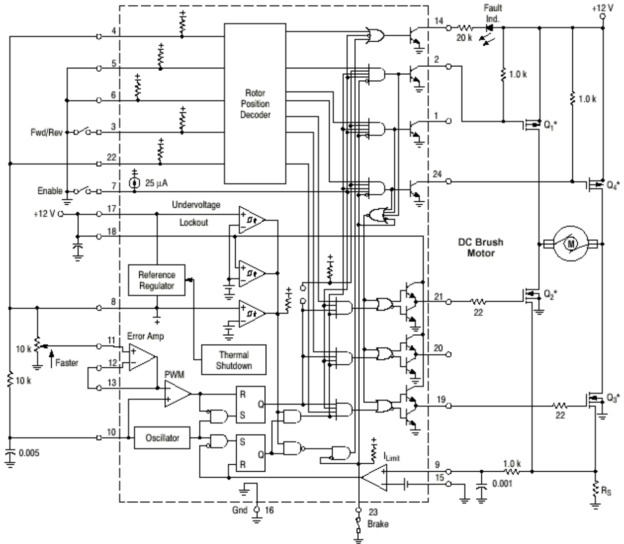
Figure 45. H-Bridge Brush-Type Controller
