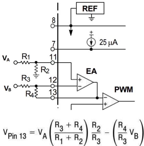
Figure 28. Current Sensing Power MOSFETs
