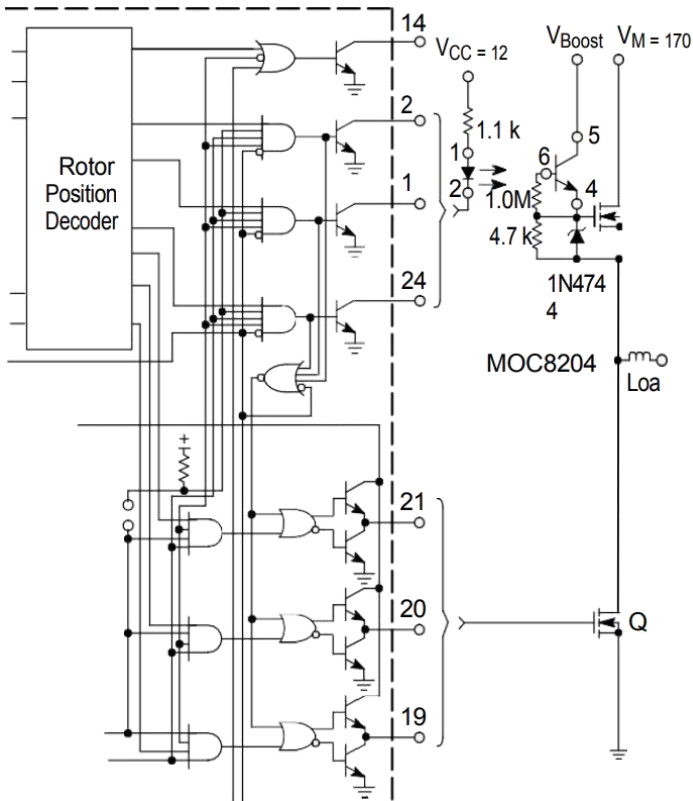
Figure 24. High Voltage Interface with N-Channel Power MOSFETs
