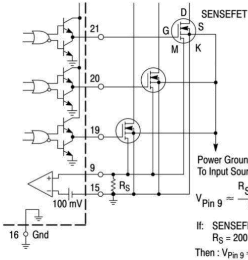
Control Circuitry Ground (Pin 16) and Current Sense Inverting Input (Pin 15) must return on separate paths to the Central Input Source Ground. Virtually lossless current sensing can be achieved with the implementation of SENSEFET power switches.
