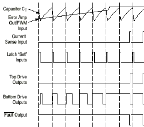
Figure 20. Pulse Width Modulator Timing Diagram Reference
