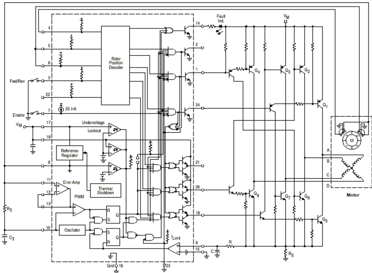
Figure 42. Four Phase, Four Step, Full Wave Motor Controller
