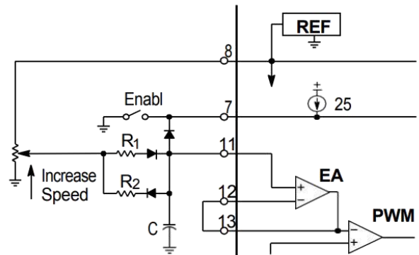
Resistor R_1 with capacitor C sets the acceleration time constant while R_2 controls the deceleration. The values of R_1 and R_2 should be at least ten times greater than the speed set potentiometer to minimize time constant variations with different speed settings.
