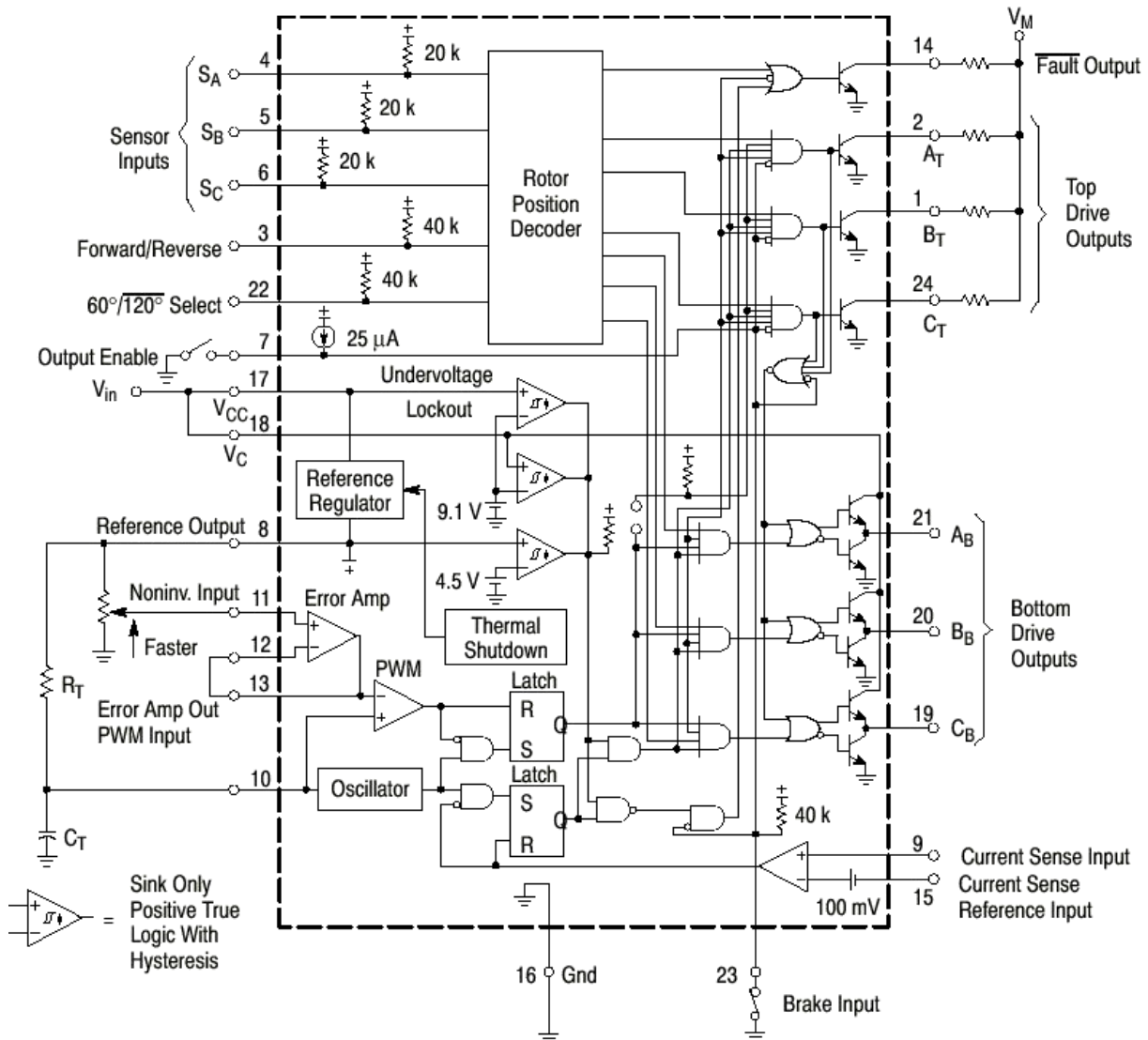
Figure 19. Block Diagram
