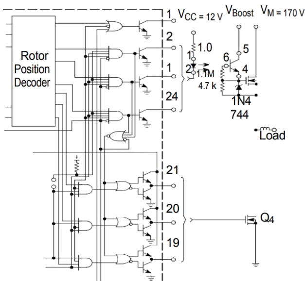
Figure 24. High Voltage Interface with N-Channel Power MOSFETs
