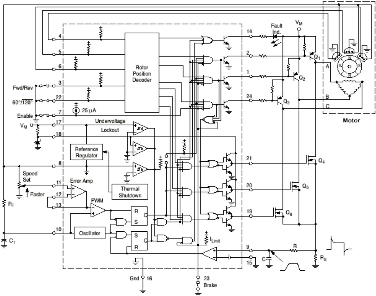
Figure 35. Three Phase, Six Step, Full Wave Motor Controller
