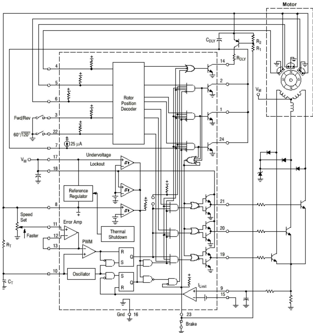
Figure 37. Three Phase, Three Step, Half Wave Motor Controller
