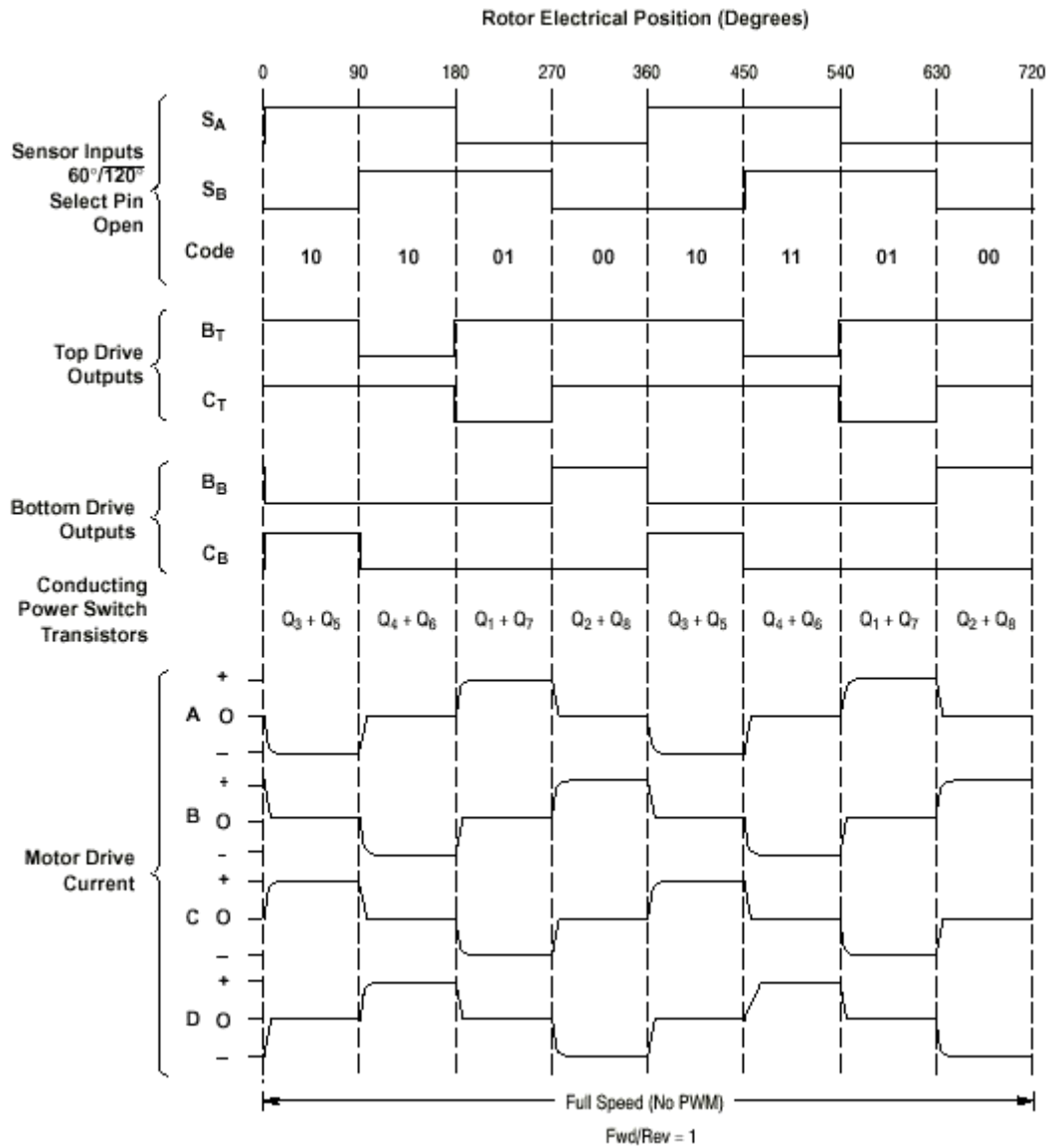
Figure 43. Four Phase, Four Step, Full Wave Motor Controller
