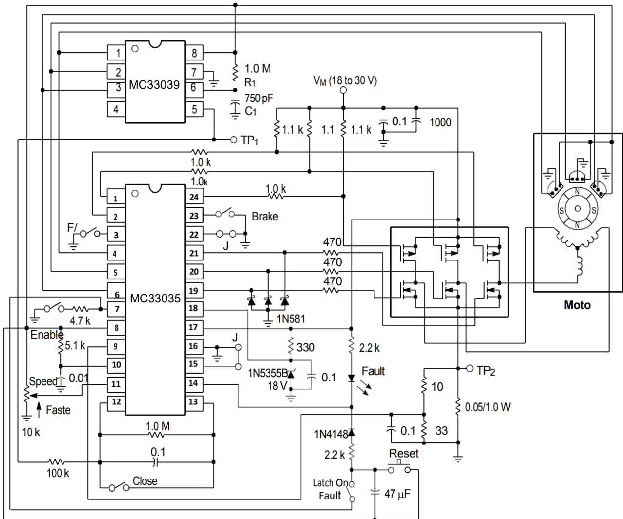
Figure 38. Closed Loop Brushless DC Motor Control Using The MC33035 and MC33039
