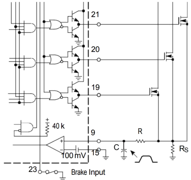
Figure 25. Current Waveform Spike Suppression
