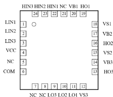
QFN-24
