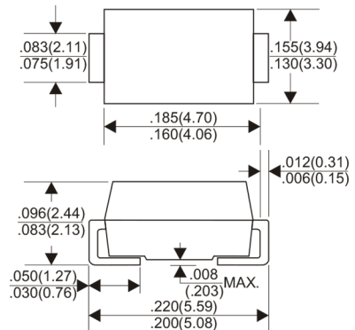
DO-214AA(SMB)
