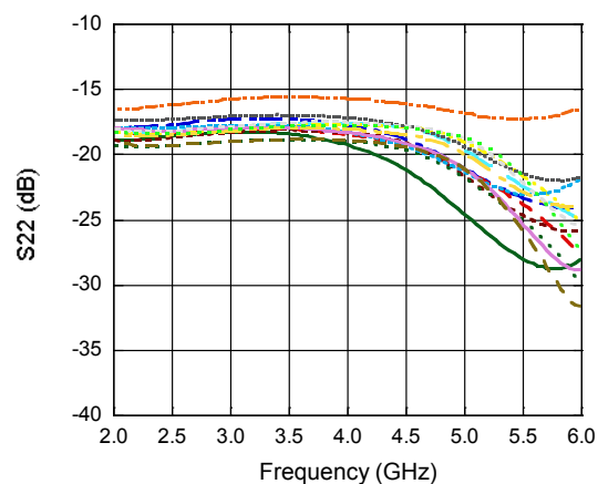
Output Return Loss, across all attenuation states
