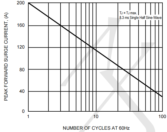
FIG. 2 - MAXIMUM NON-REPETITIVE
