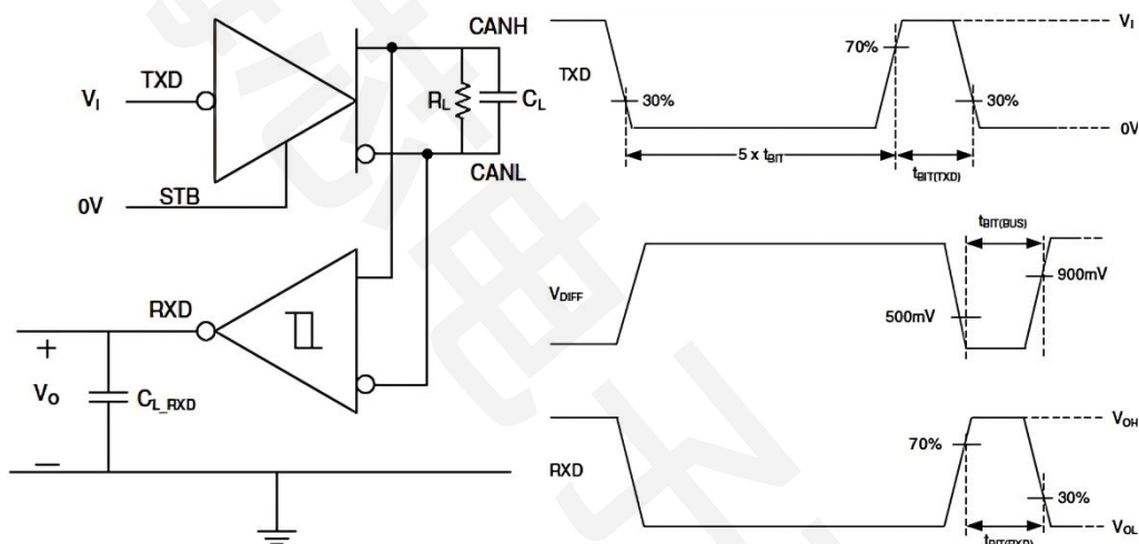
CAN FD Timing Parameter Measurement
