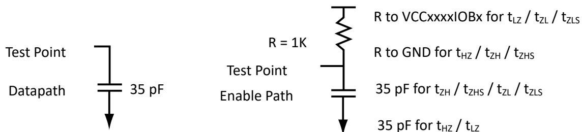
Figure 5-8. AC Loading
