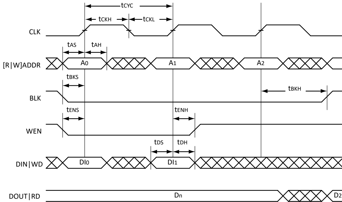
Figure 11-4. RAM Write, Output Retained. Applicable to both RAM4K9 and RAM512x18
