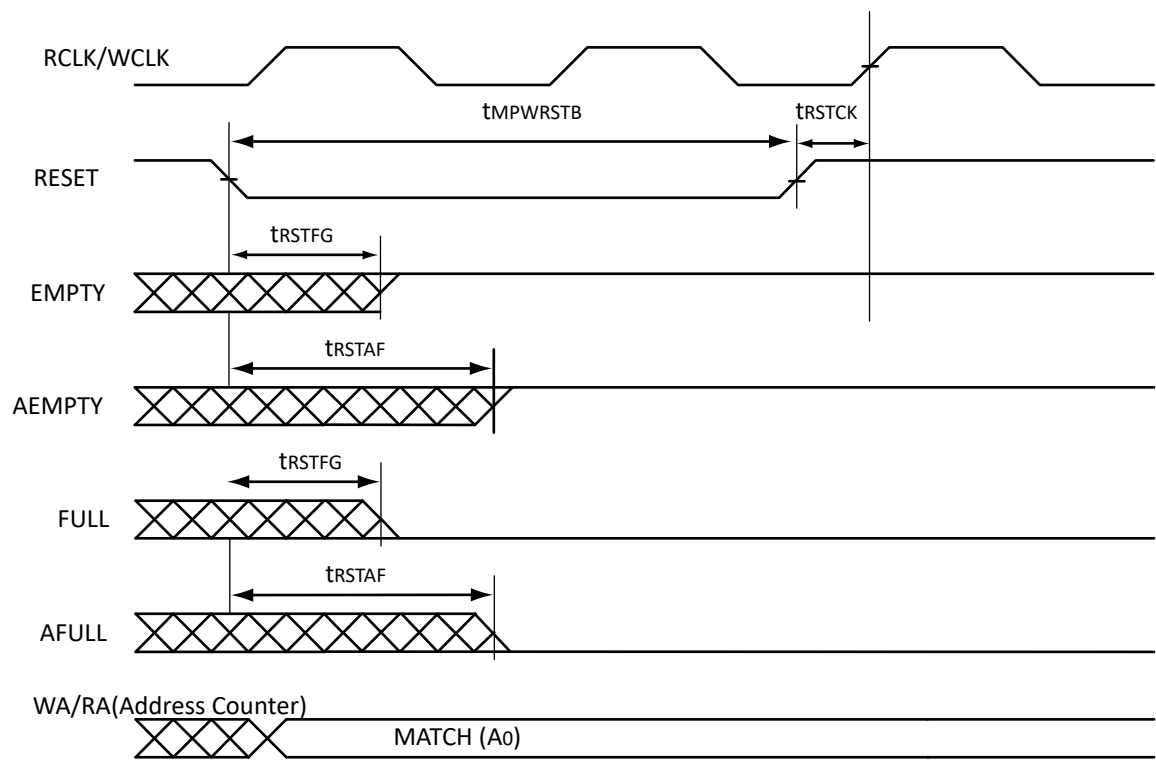
Figure 11-10. FIFO Reset
