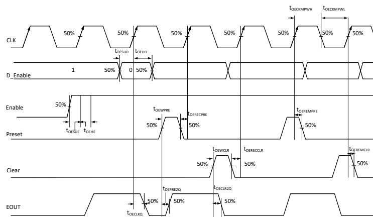
Figure 5-17. Output Enable Register Timing Diagram
