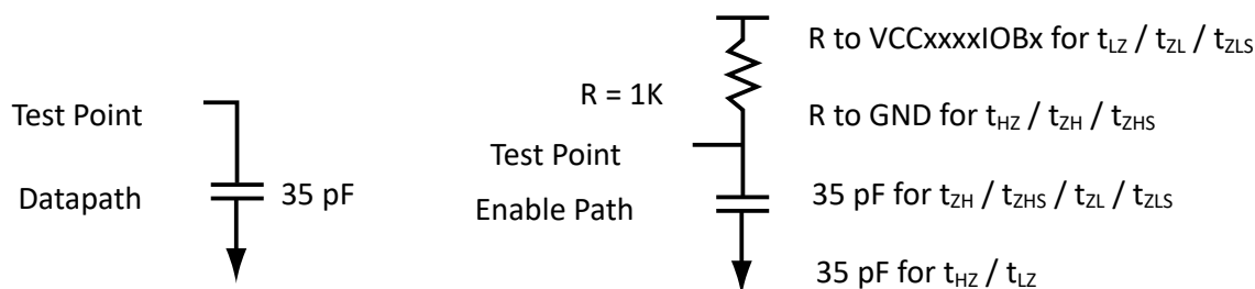
Figure 5-6. AC Loading
