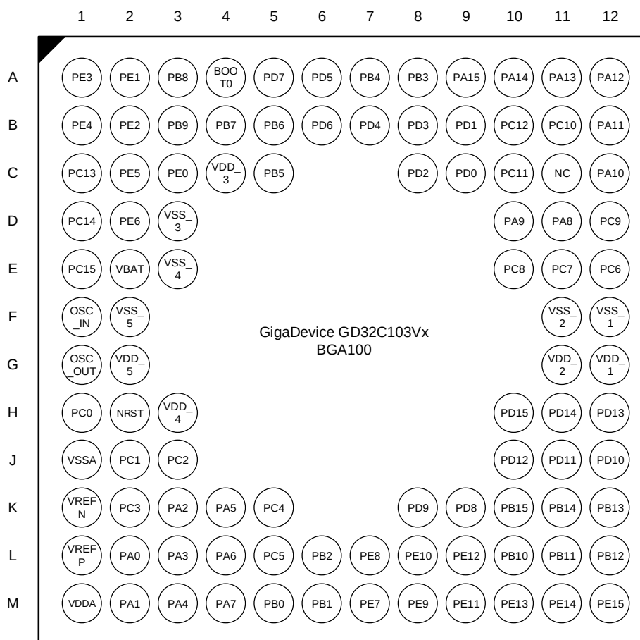
Figure 2-2. GD32C103Vx BGA100 pinouts
