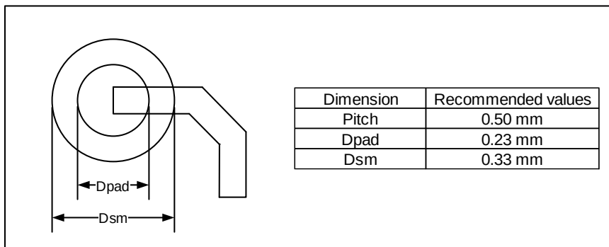
Figure 5-4. BGA100 recommended footprint
