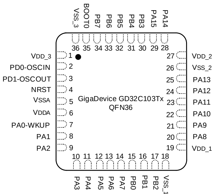
Figure 2-6. GD32C103Tx QFN36 pinouts
