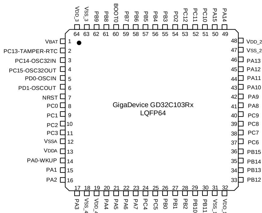
Figure 2-4. GD32C103Rx LQFP64 pinouts
