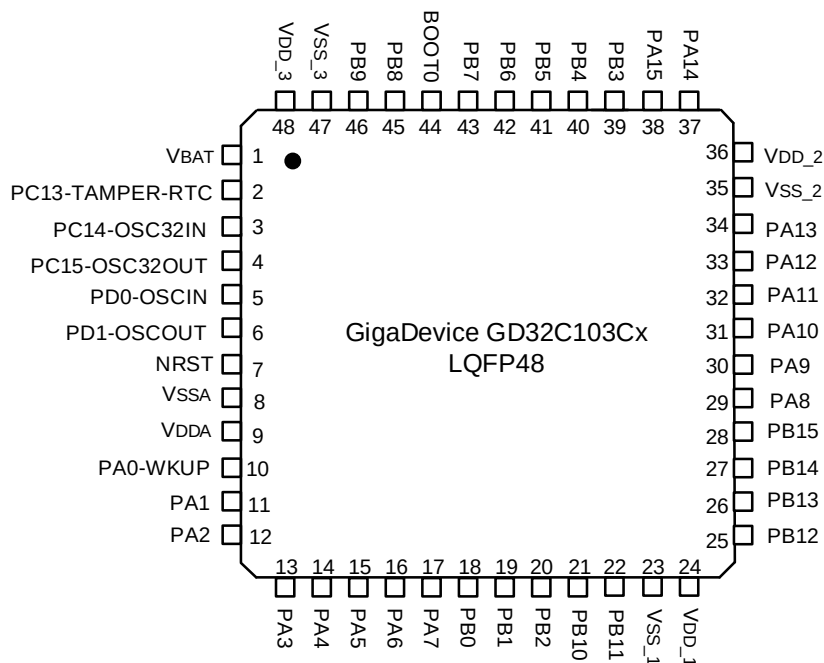
Figure 2-5. GD32C103Cx LQFP48 pinouts
