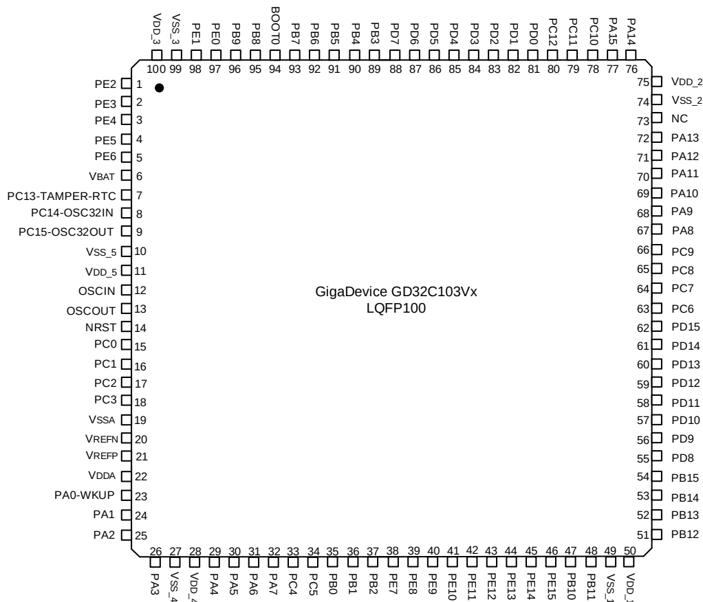
Figure 2-3. GD32C103Vx LQFP100 pinouts
