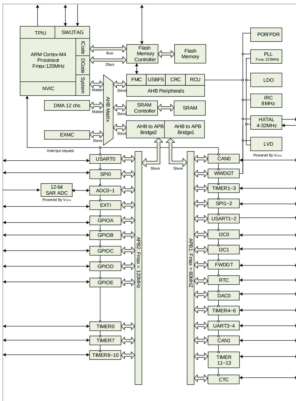
Figure 2-1.GD32C103xx block diagram
