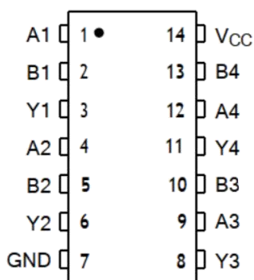
Figure 1. Pin Assignment
