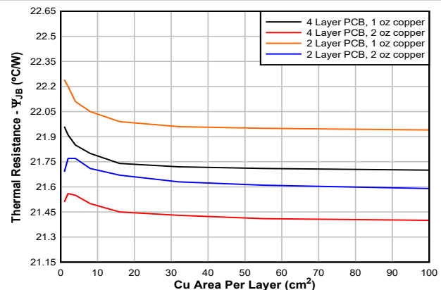
Figure 8-9. \psi_{JB} vs Copper Area (DYB Package)
