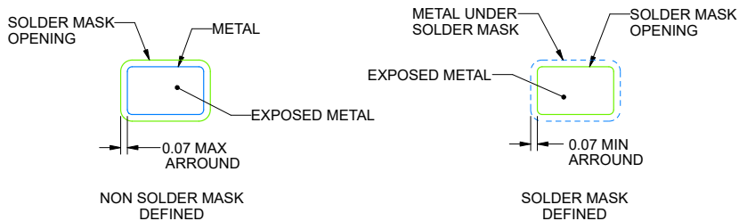
SOLDERMASK DETAILS
