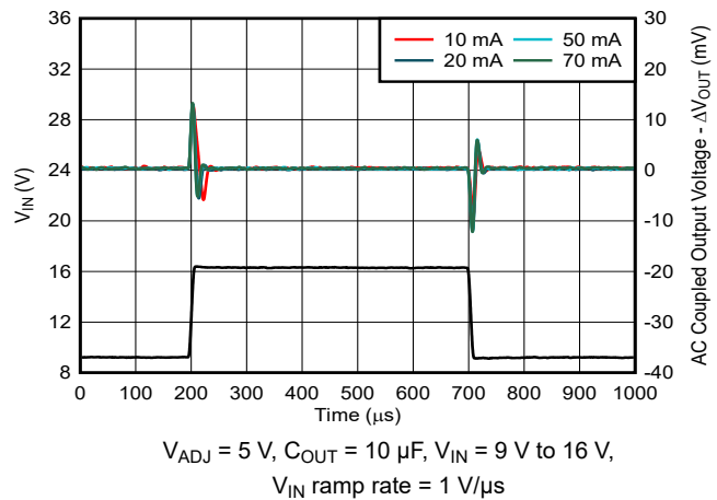
Figure 6-18. Line Transient
