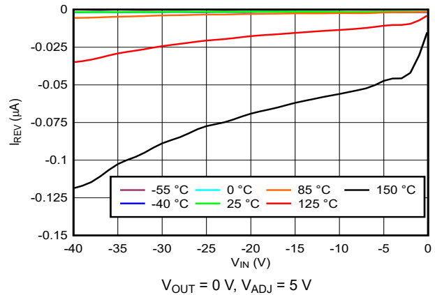
Figure 6-16. Reverse Current vs Input Voltage
