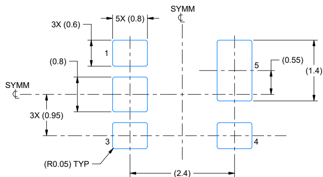
LAND PATTERN EXAMPLE EXPLODED METAL SHOWN SCALE:15X
