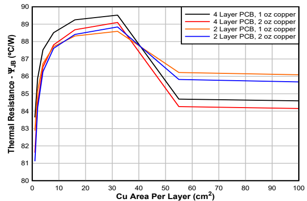
Figure 8-7. \psi_{JB} vs Copper Area (DBV Package)
