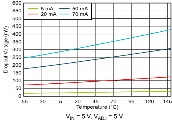
Figure 6-7. Dropout Voltage vs Ambient Temperature
