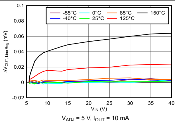
Figure 6-4. Line Regulation
