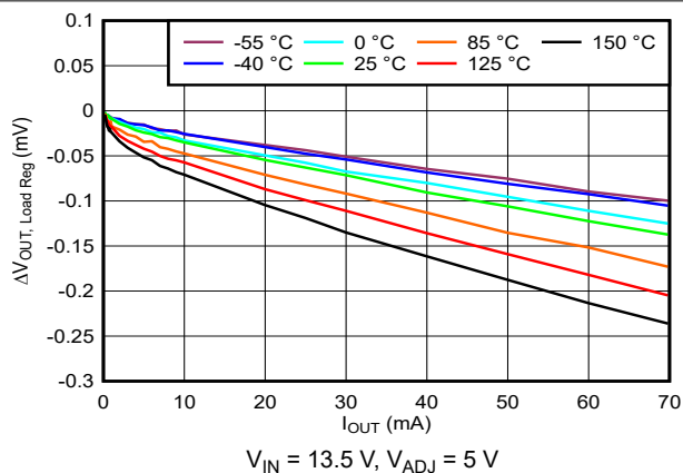
Figure 6-2. Load Regulation
