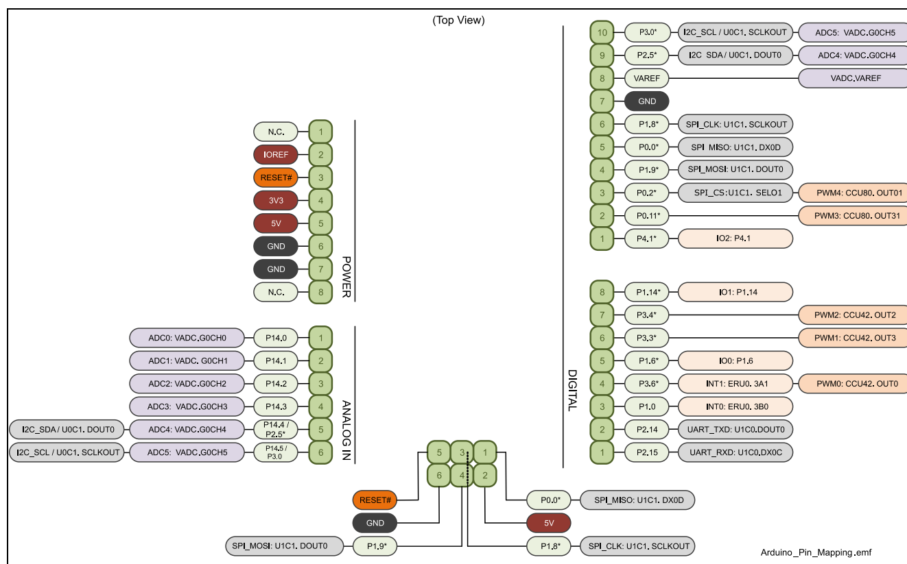
Figure 9 Mapping of Arduino Functions to XMC Pin Functions
