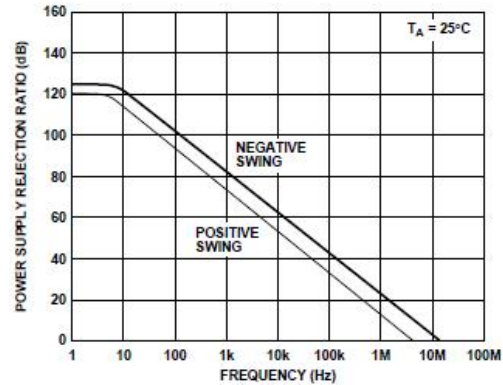
Figure 29. PSRR vs. Frequency
