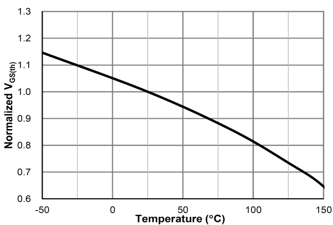
V_{GS(th)} vs. Junction Temperature
