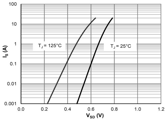
Body-Diode Characteristics
