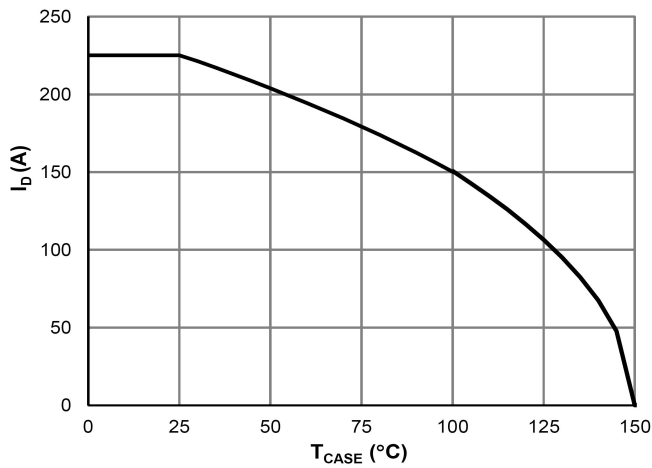
Current De-rating
