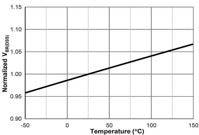
V_{BR(DSS)} vs. Junction Temperature
