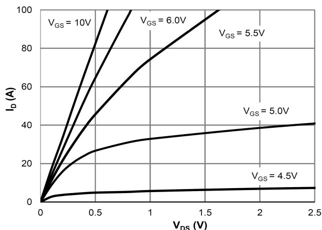
Saturation Characteristics
