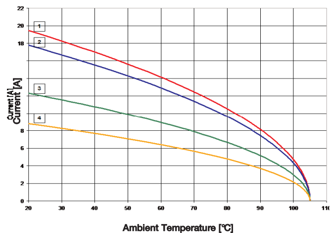
Current rating - SURE-SEAL
