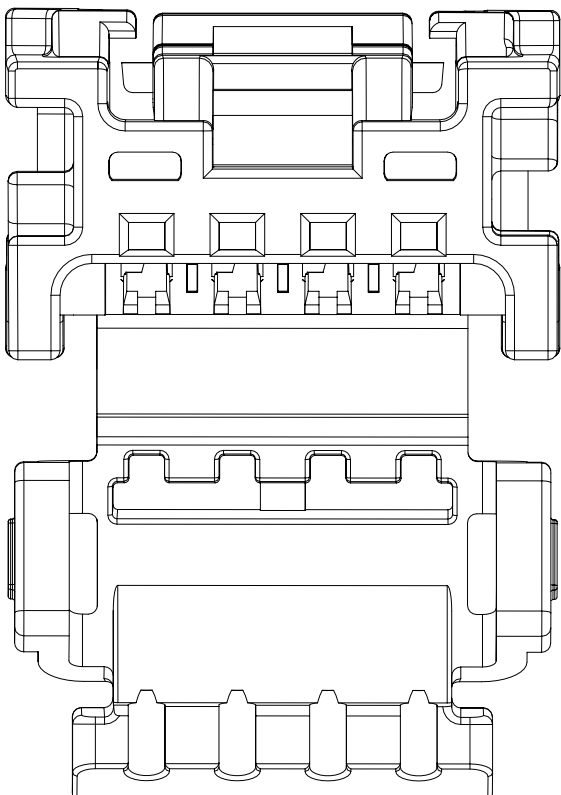
4 CIRCUIT RECEPTACLE NO BRIDGE POLARIZATION OPTION D
