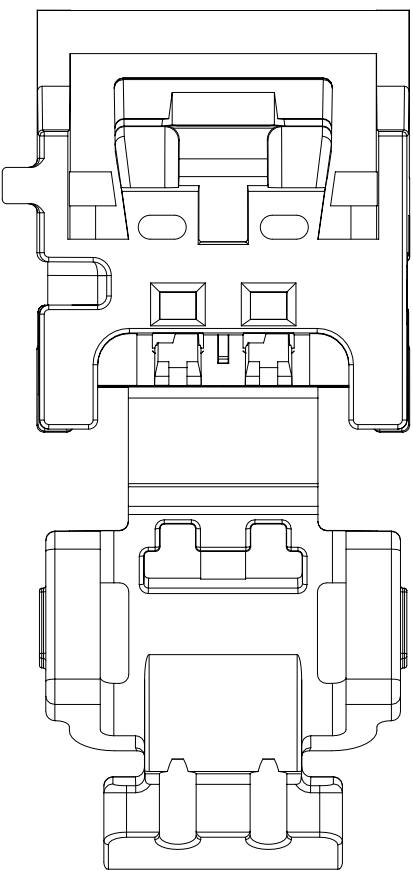
2 CIRCUIT RECEPTACLE BRIDGED POLARIZATION OPTION B
