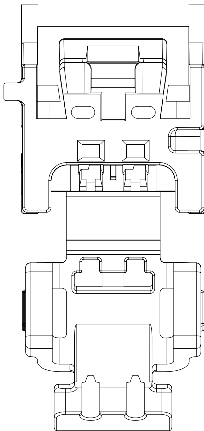
2 CIRCUIT RECEPTACLE BRIDGED POLARIZATION OPTION D
