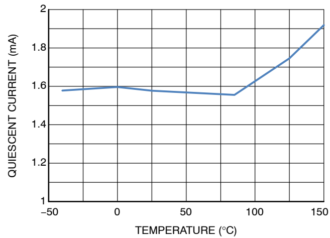
Figure 22. Quiescent Current
