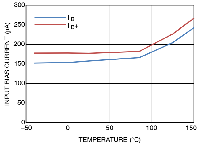
Figure 8. Preamplifier Input Bias Current vs. Temperature
