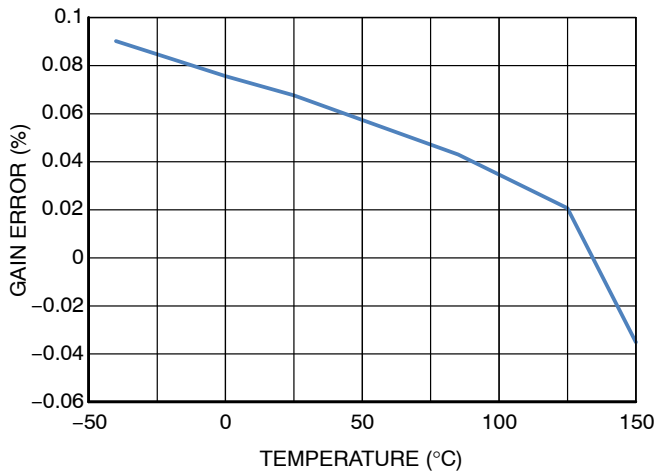
Figure 9. Preamplifier Gain Error vs. Temperature
