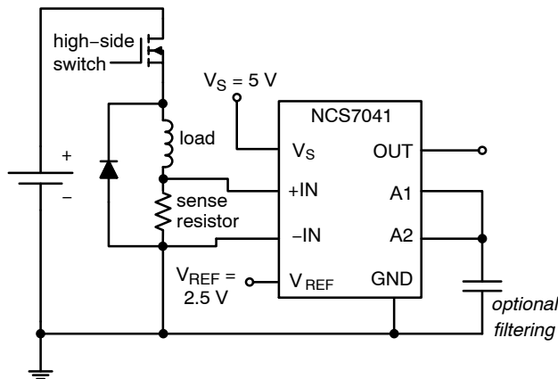
Figure 23. Low-side Current Sensing
