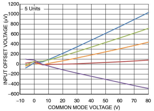
Figure 6. Input Offset Voltage vs. Common Mode Input Voltage
