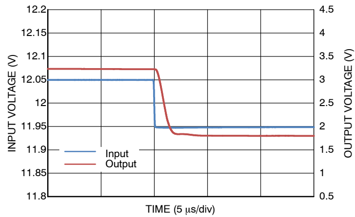
Figure 19. Transient Response
