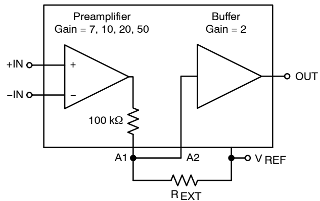
Figure 26. Lowering the Gain Using an External Resistor
