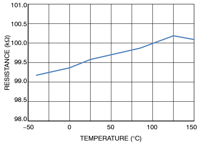
Figure 10. Preamplifier Output Resistance vs. Temperature
