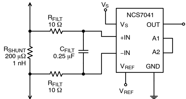
Figure 30. Input Filtering Compensates for Shunt Inductance on Shunts Less than 1 mΩ, as Well as High Frequency Noise in Any Application
