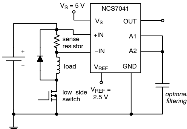
Figure 24. High-side Current Sensing
