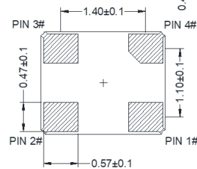
[底部视图]
