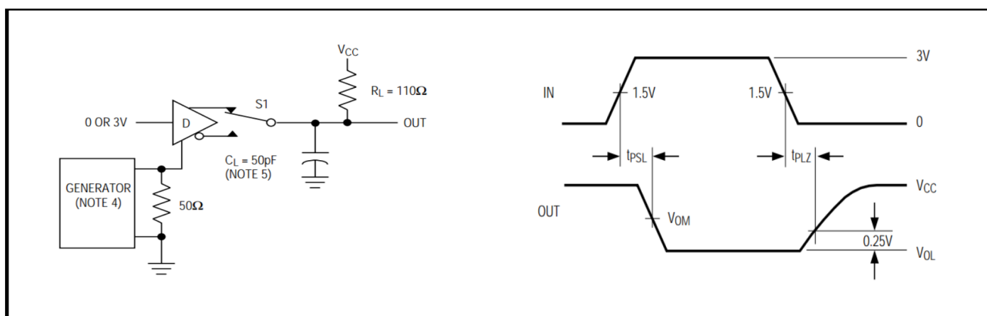
Figure 6 Driver enable and disable time
