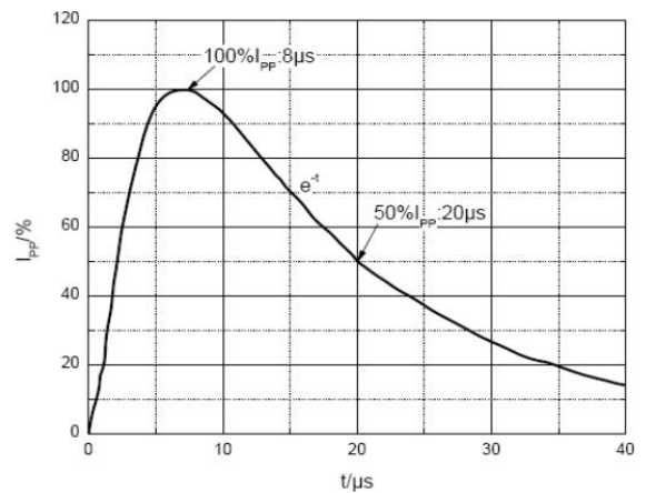
8/20µs pulse waveform according to IEC 61000-4-
