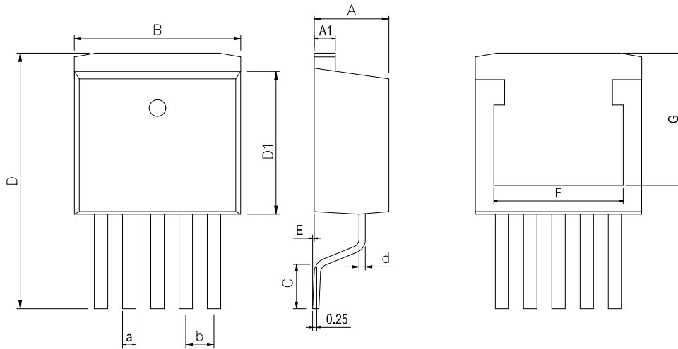
Dimensions In Millimeters(TO-263-5)
