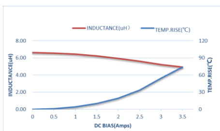
ZETC303015D6R8MBT-LF
