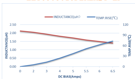
ZETC303015D2R2MBT-LF
