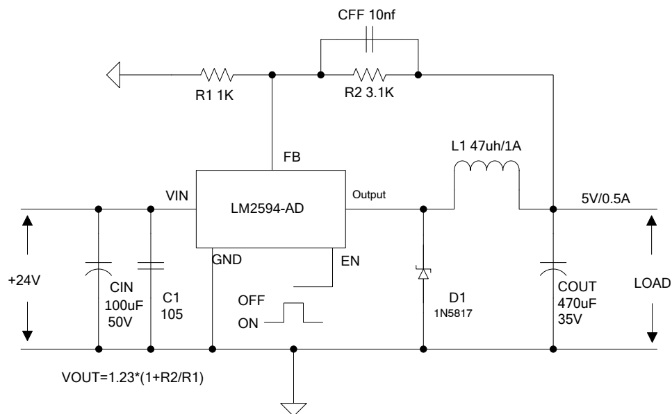
Figure8. LM2594-AD System Parameters Test Circuit
