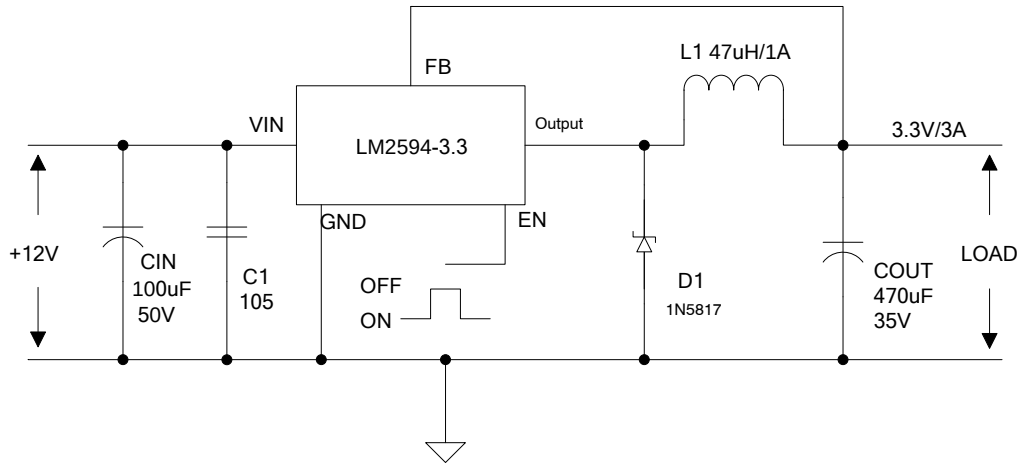
Figure5. LM2594-3.3 System Parameters Test Circuit
