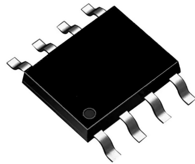
Figure 1. Package Types of LM2594
