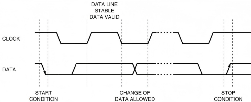
Figure: Serial bus data transfer
