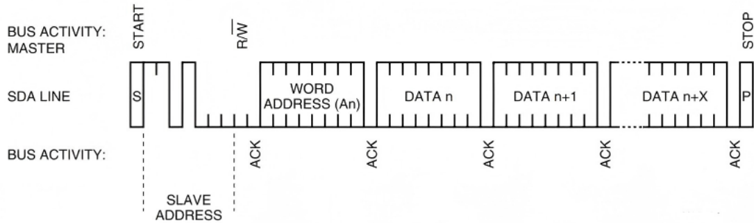
Figure: Write mode sequence
