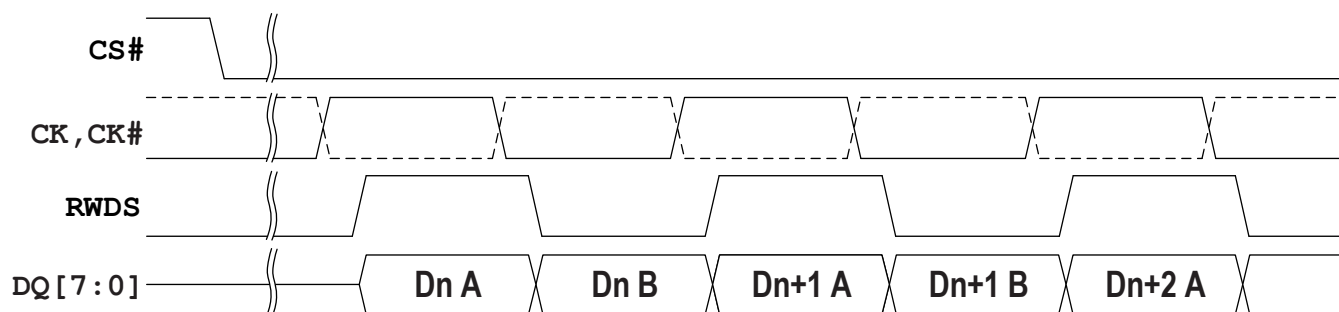
Figure 6 - Data Placement during a Read Transaction
