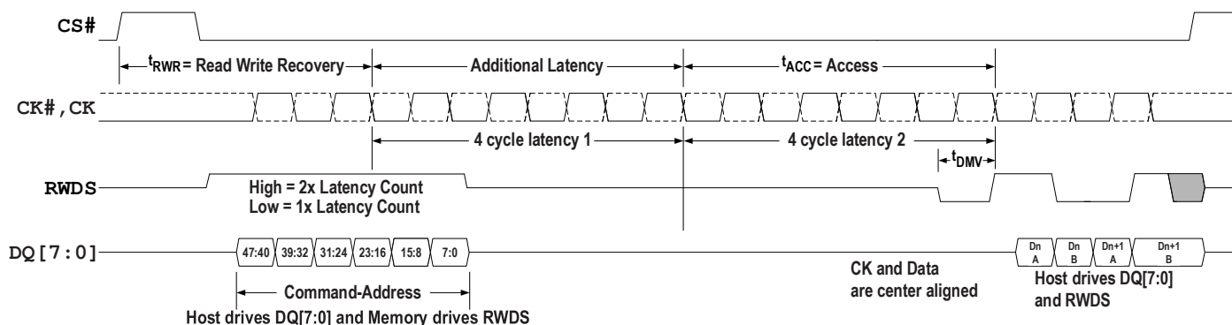
Figure 31 - Write Timing Diagram — With Additional Latency
