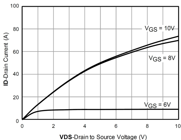
Output Characteristics; typical values
