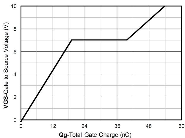
Gate Charge; typical values
