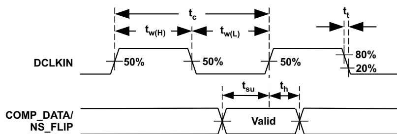
图 3. Control Timing
