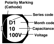
Fig.1 ΦD=4~10mm
