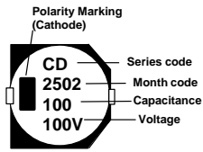
Fig.2 ΦD≥12.5mm
