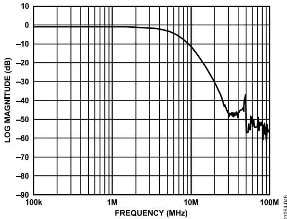
Figure 47. Video Filter Response
