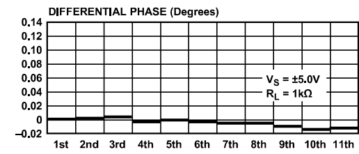
Figure 34. Differential Gain and Differential Phase One Back Terminated Load (150 Ω) (Video Op Amps Only)
