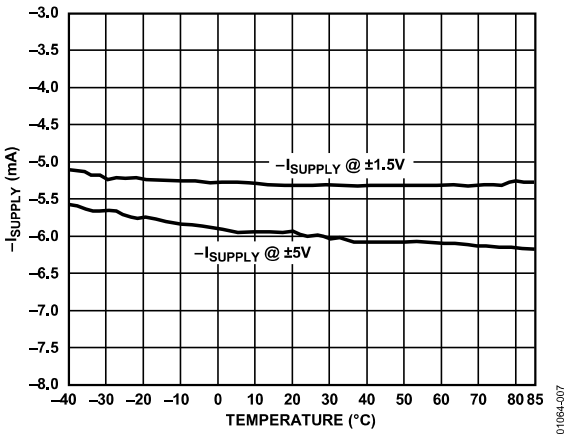
Figure 7. -I_{SUPPLY} vs. Temperature
