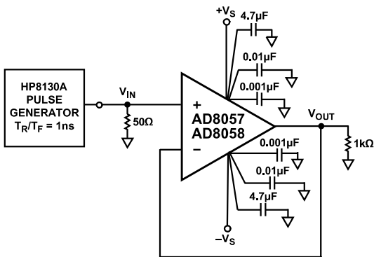
Figure 41. Test Circuit, G = +1 , R_L = 1\text{ k}\Omega
