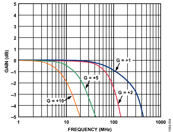
Figure 4. Small Signal Frequency Response
