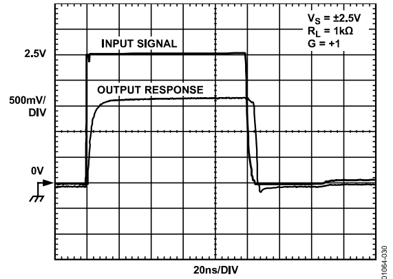
Figure 28. Input Overload Recovery, V_S = \pm 2.5 V
