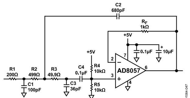
Figure 46. Low-Pass Filter for Video
