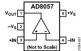
Figure 1. RT-5 (SOT-23)
