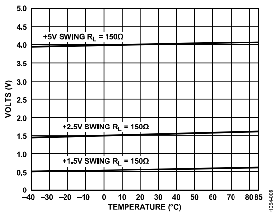
Figure 8. Positive Output Voltage Swing vs. Temperature
