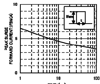
IFSM-t CHARACTERISTICS
