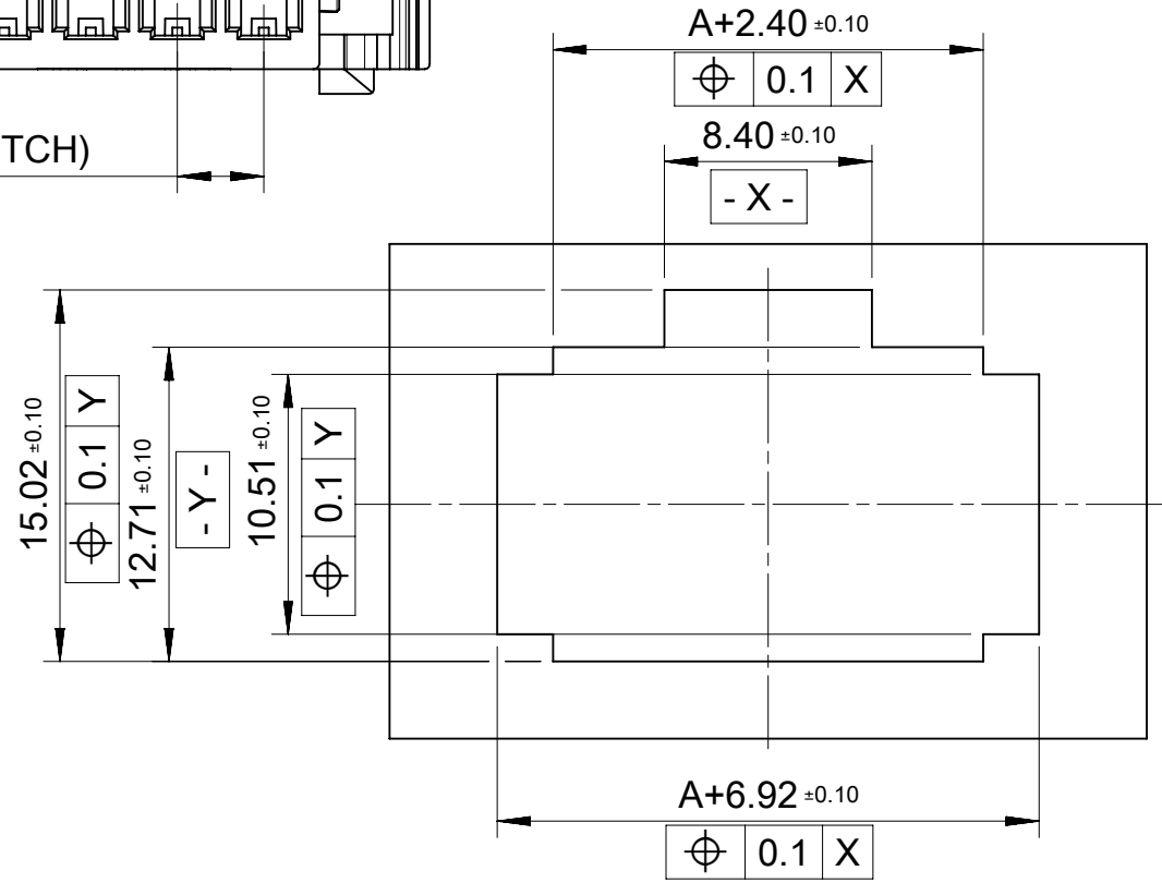
RECOMMENDED PANEL CUT OUT (TOLERRANCE +/-0.05 THICKNESS=1.2~2.0MM)
