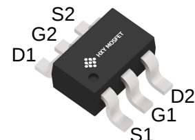
SOT-363 (SOT-363-6)
