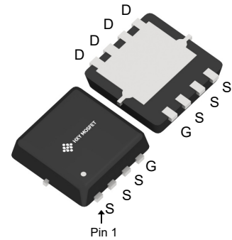
DFN3X3-8L (DFN-8(3.3x3.3))
