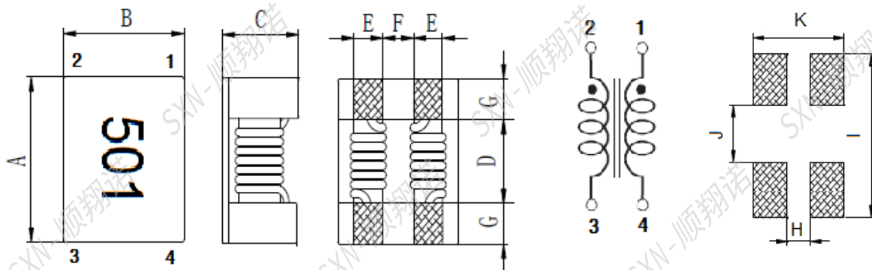
Schematic
