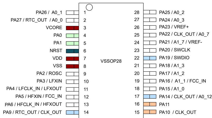
Figure 6-7. 28-Pin DGS28(VSSOP) (Top View)
