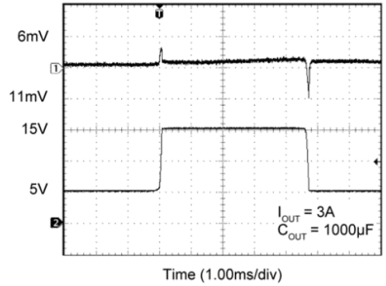
MIC29302AW Line Transient Response with 3A Load, 1000µF Output Capacitance
